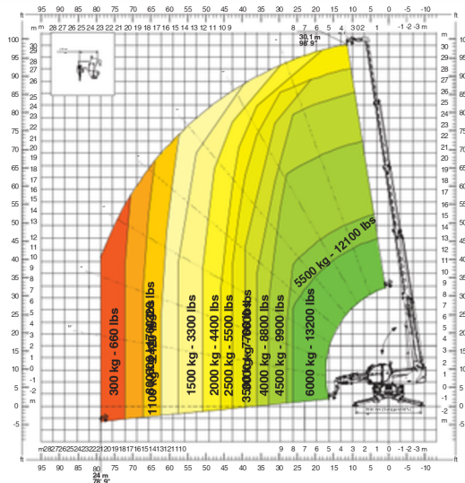
HOOK 6,000 kg
