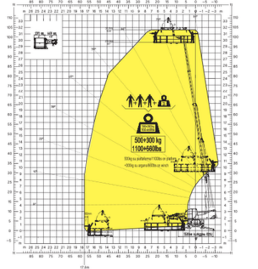
BASKET 6,5 m WITH WINCH 500 kg 300 kg
