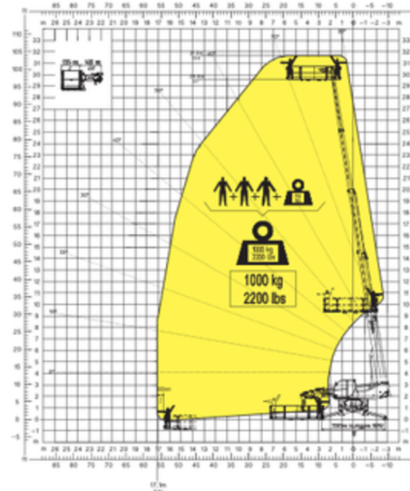
ROTATING EXTENDABLE BASKET 1,000kg
