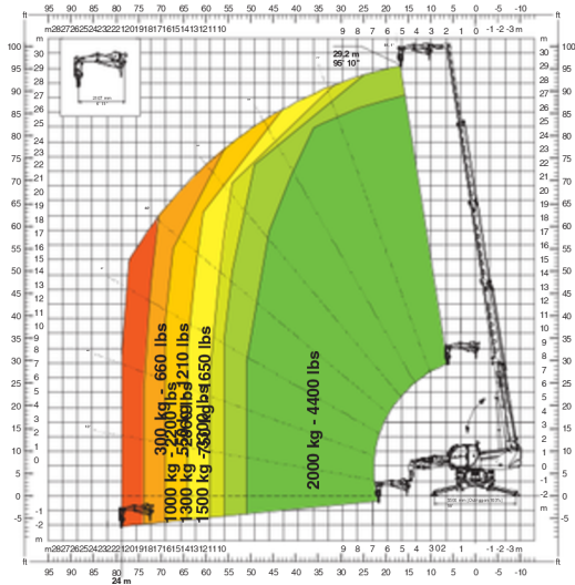
JIB WITH WINCH 2,000 kg
