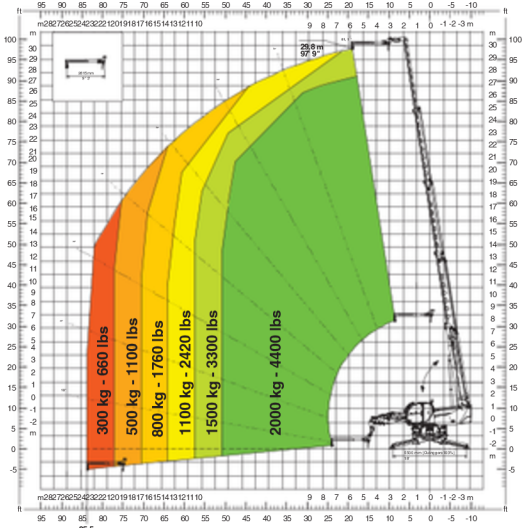
JIB 2,000 kg
