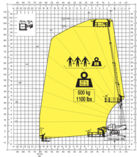
ROTATING EXTENDABLE BASKET 500 kg
